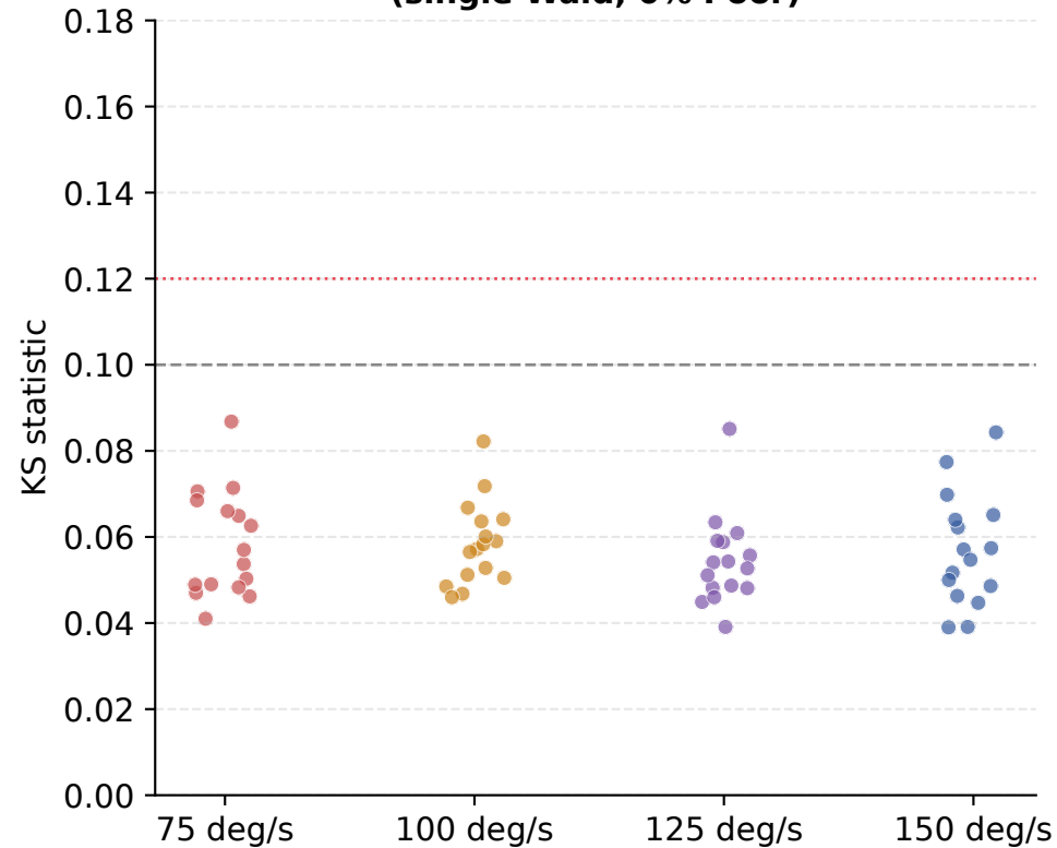
A. HRT fit quality (single-Wald, 0% Poor)
