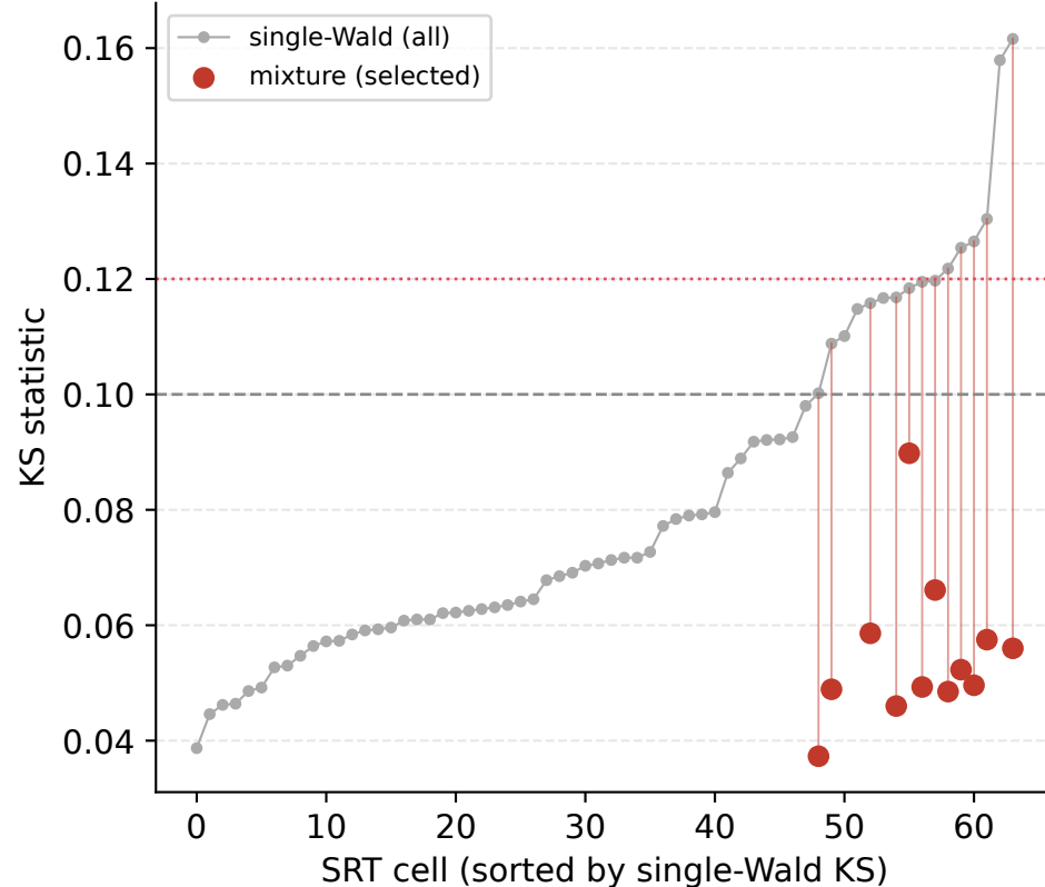
B. SRT fit quality (mixture rescues bimodal cells)
