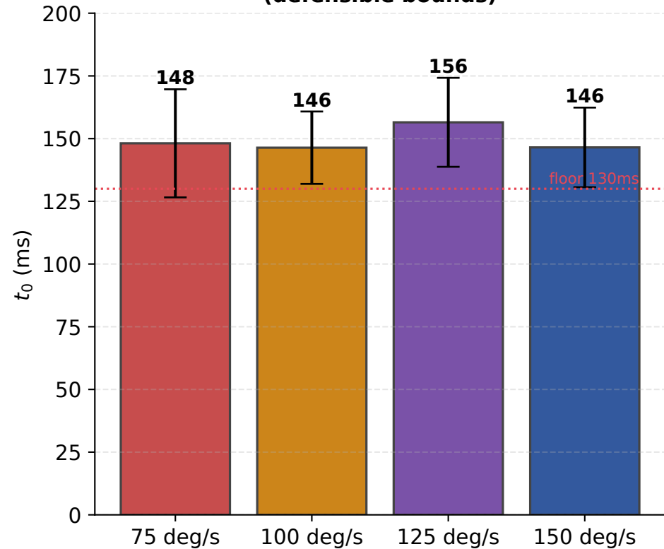
C. HRT non-decision time (defensible bounds)
